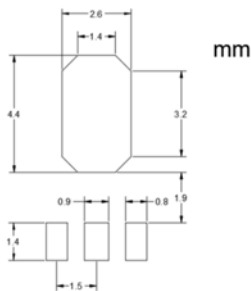
SOT-89 Suggested Pad Layout
